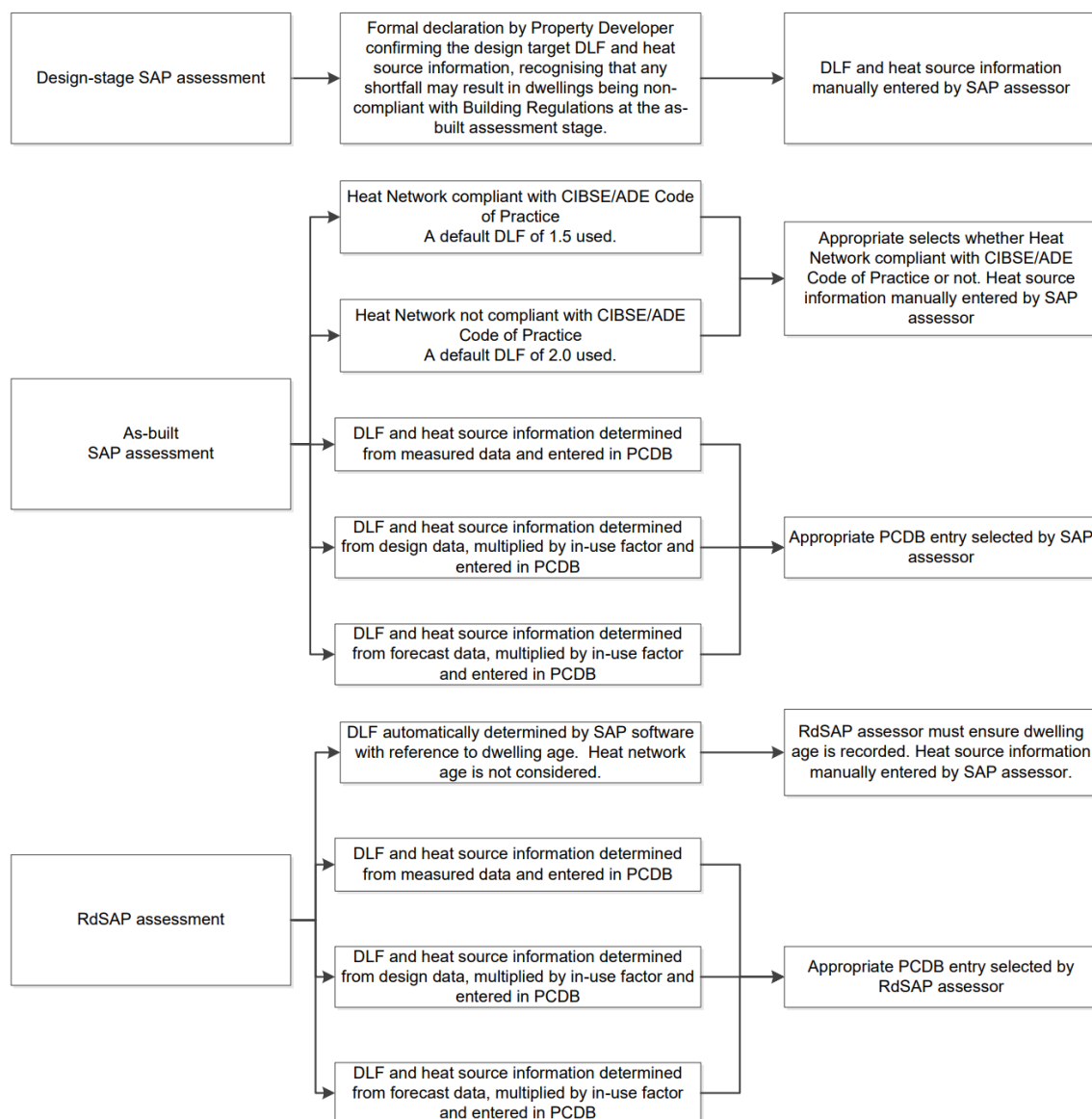
Figure 2- SAP Heat network input process
